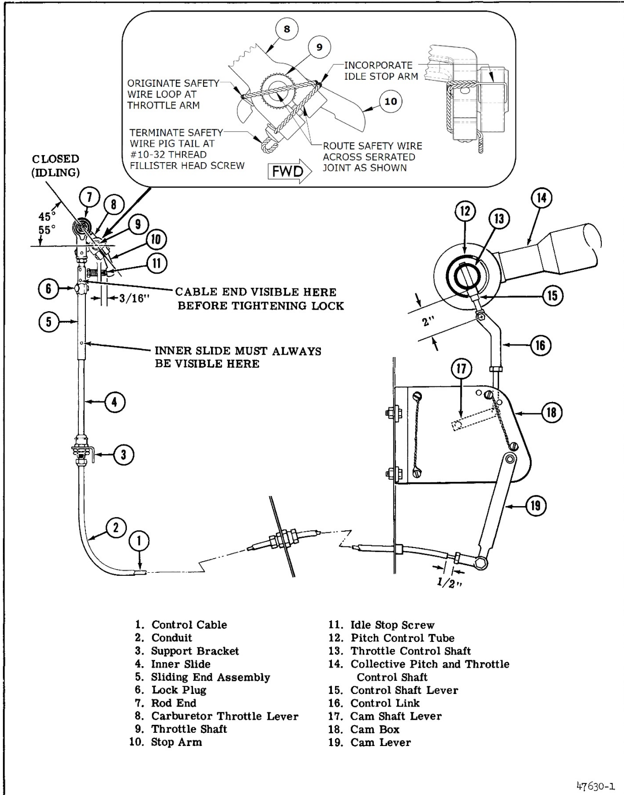
Figure 3-11. Throttle Linkage Adjustment
