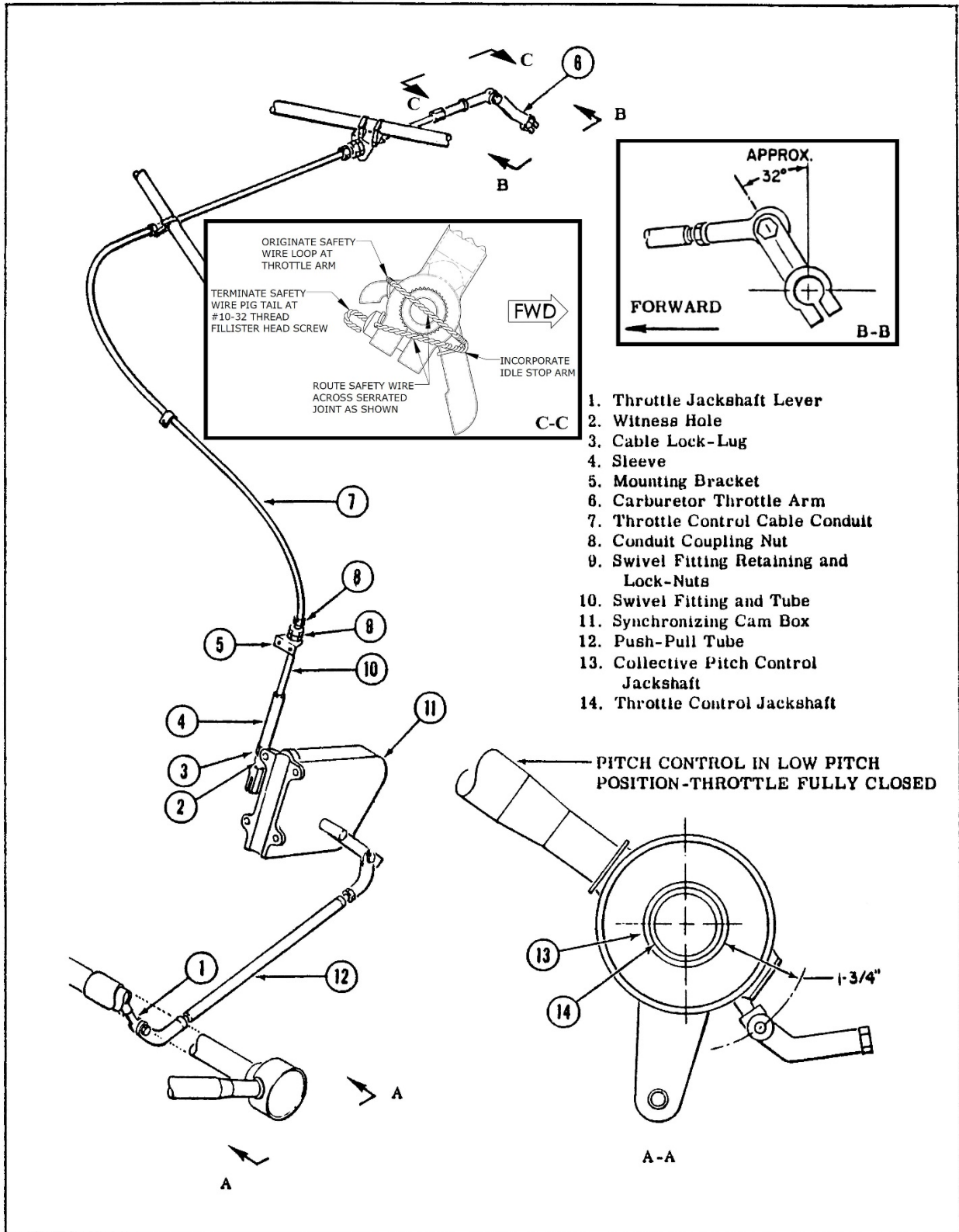
Figure 3-13. Adjusting Throttle Linkage
