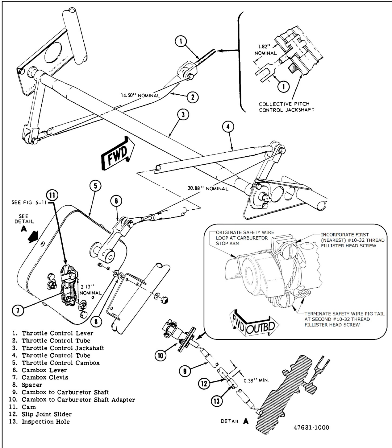
Figure 5-10. Throttle Control Installation (Sheet 1 of 2)
