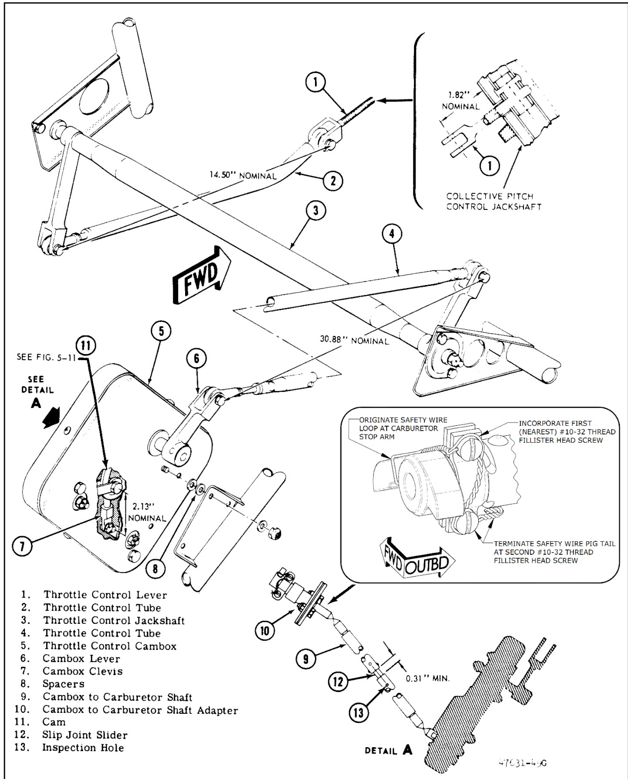
Figure 5-10. Throttle Control Installation
